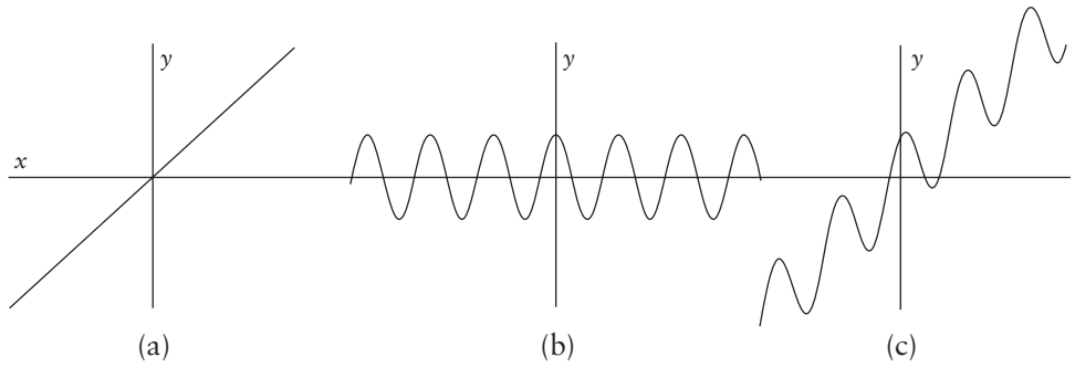
FIGURE 20.34 (a) The undistorted domain y = x , (b) a distortion function y = \cos(x) , and (c) the distorted domain y = x + \cos(x) .
