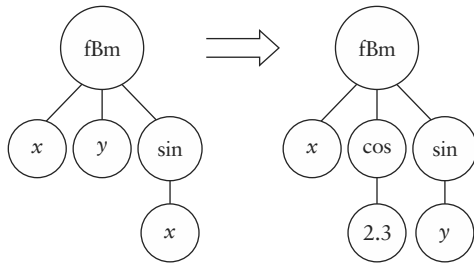
FIGURE 19.2 Mutation in an expression tree.
