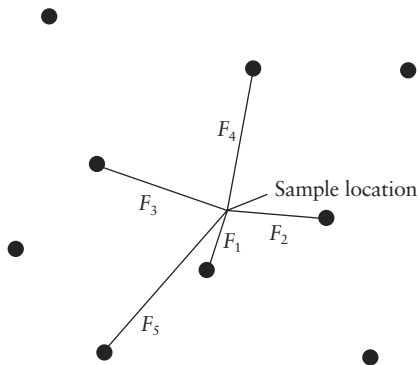
FIGURE 4.1 F_n values are the distance to the n th closest feature point.
